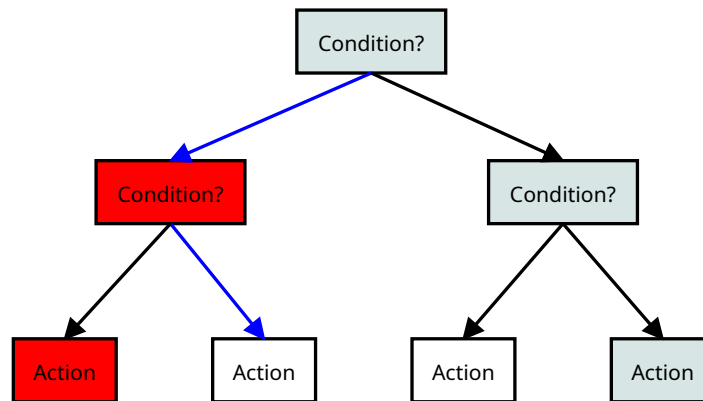
Figure 341: Example of a behaviour tree
